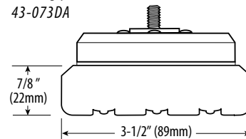
Backing plate 43-073DA
