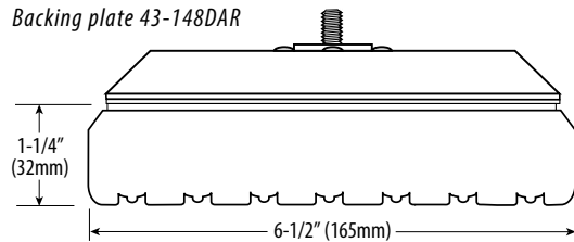
Backing plate 43-148DAR
